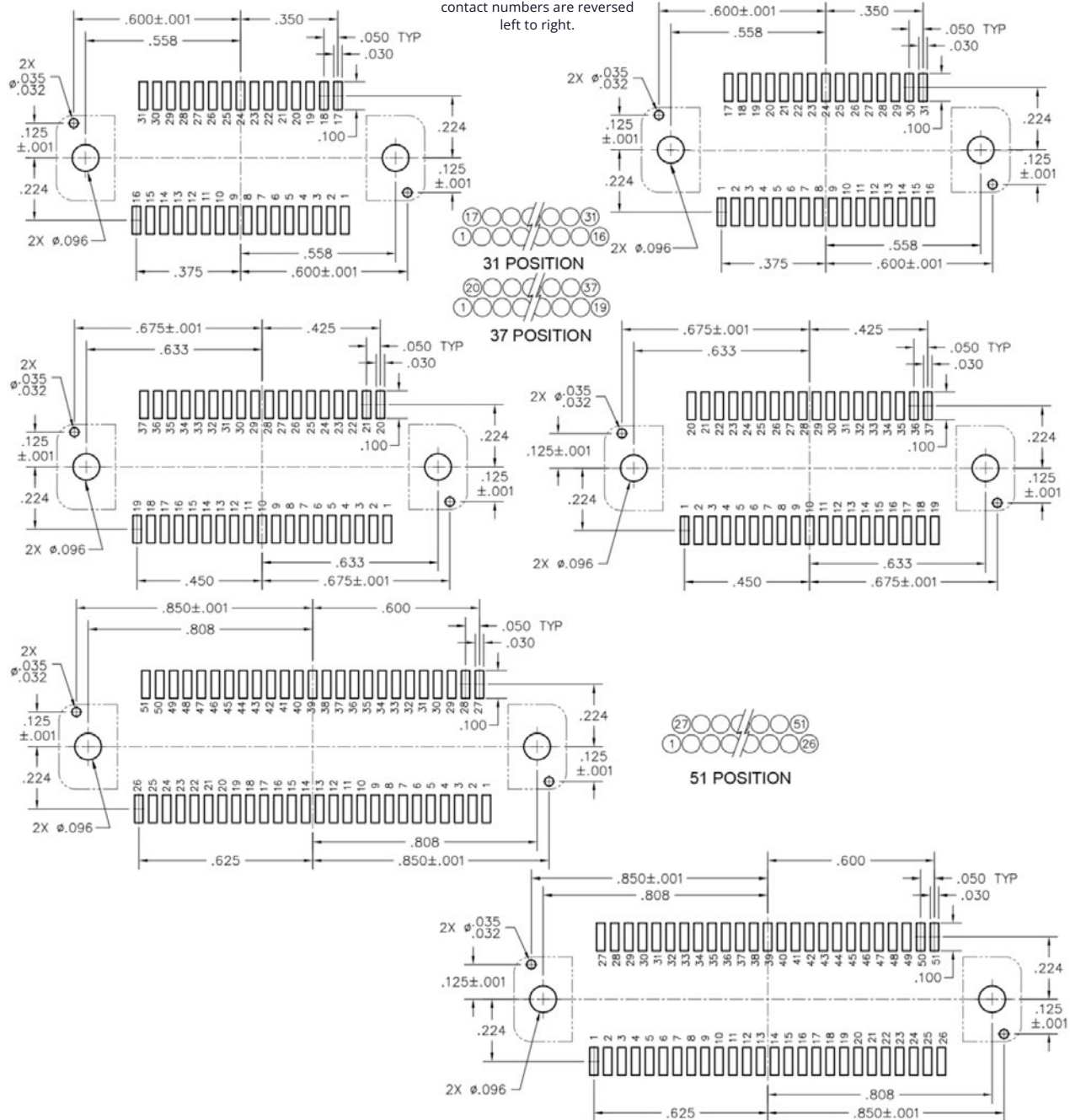
CONNECTOR MATING FACE* (RECEPTACLE)
