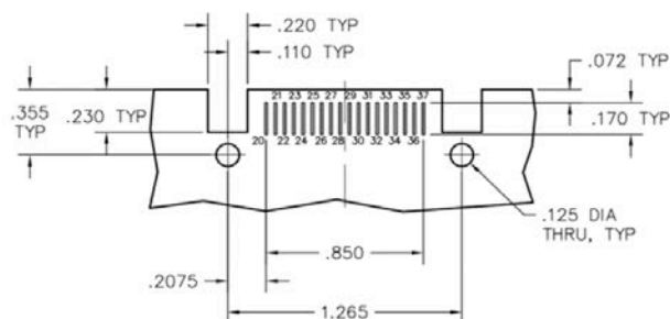
PLUG PC BOARD LAYOUT COMPONENT SIDE
