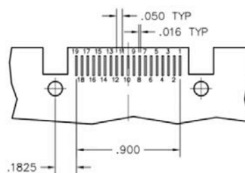
PLUG PC BOARD LAYOUT CIRCUIT SIDE
