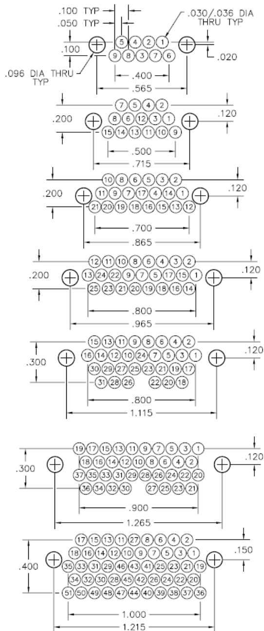
PC BOARD LAYOUT COMPONENT SIDE
