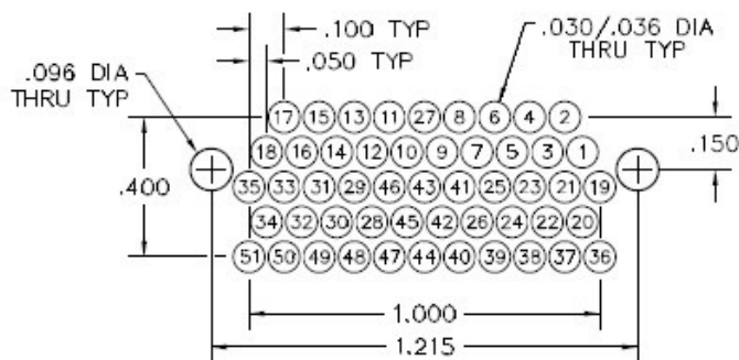
PC BOARD LAYOUT COMPONENT SIDE
