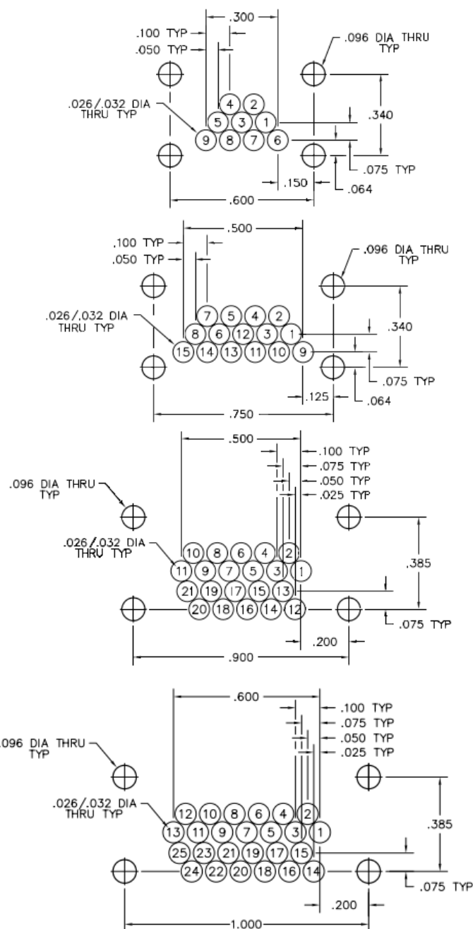
PC BOARD LAYOUT COMPONENT SIDE
